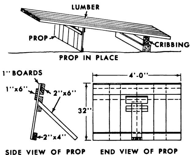
Figure 11-2. Lumber props.
